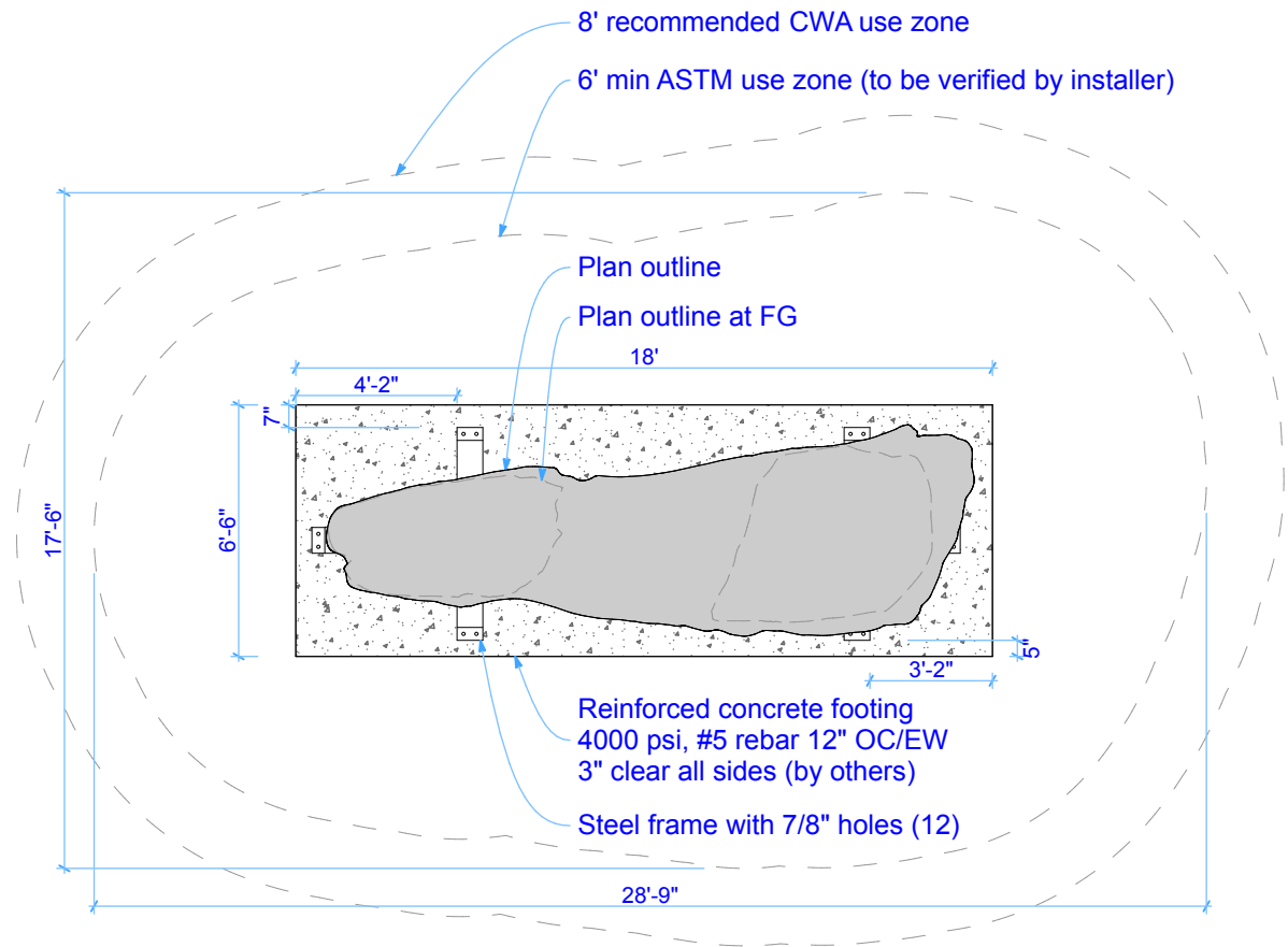
1 Plan SCALE: 3/16" = 1'-0"
