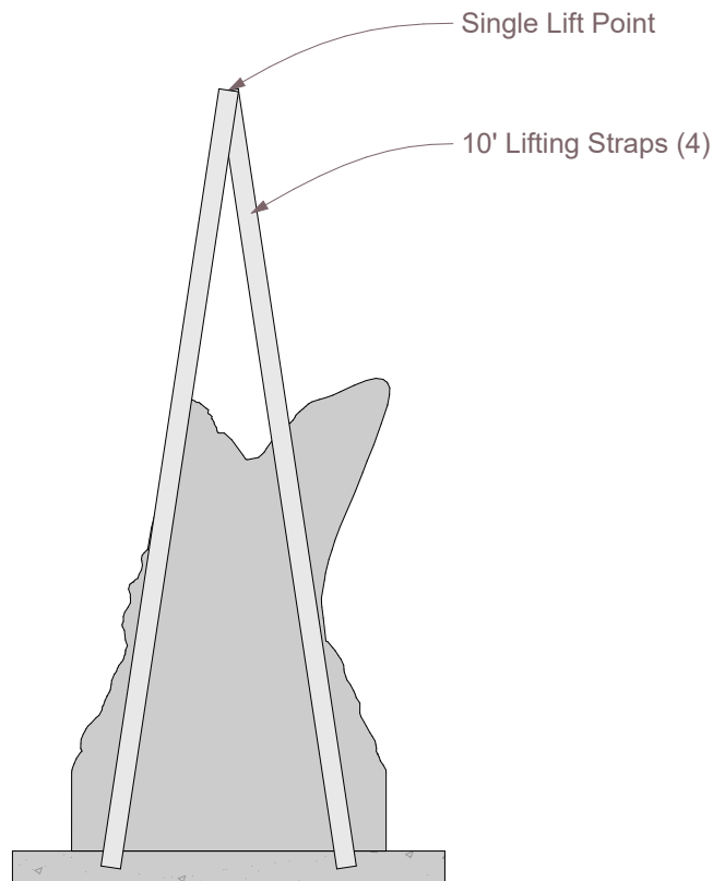
Pick Diagram - Elevation
