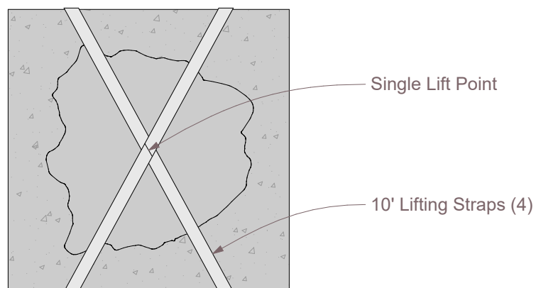
Pick Diagram - Plan
