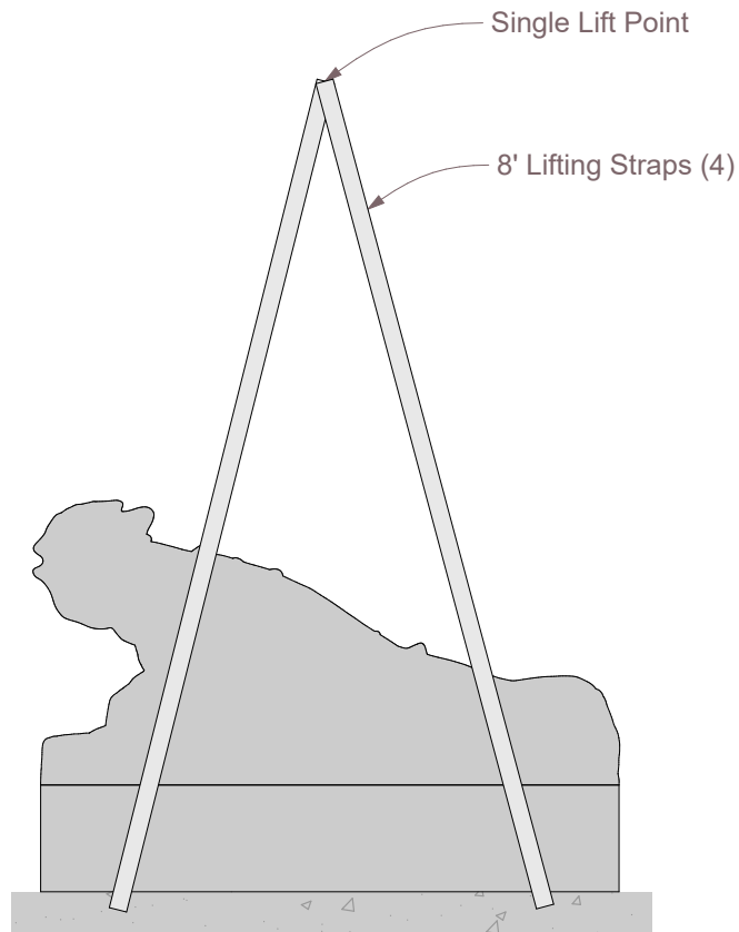
Pick Diagram - Elevation
