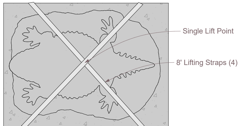
Pick Diagram - Plan
