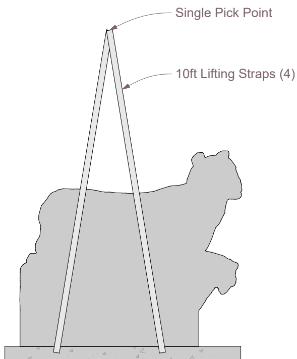
Pick Diagram - Elevation
