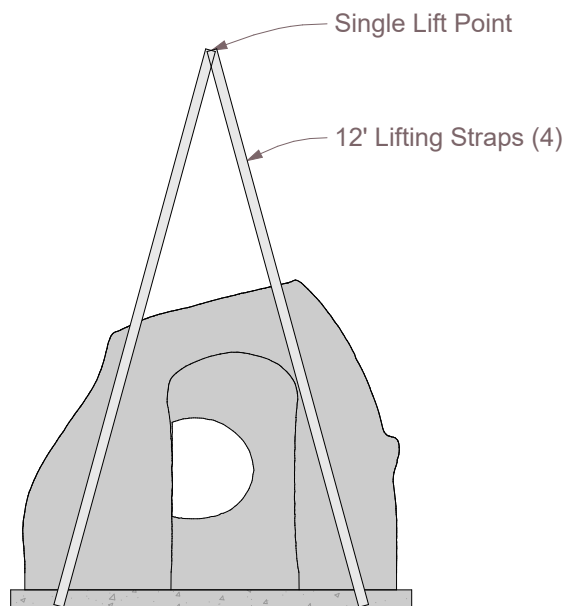
Pick Diagram - Elevation
