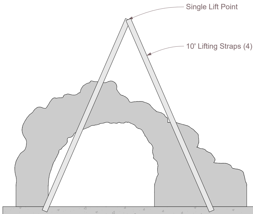
Pick Diagram - Elevation
