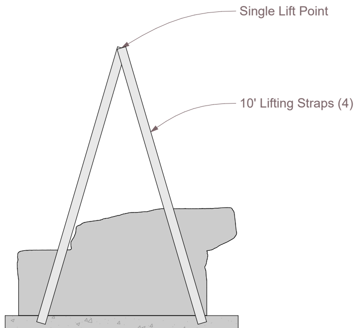
Pick Diagram - Elevation
