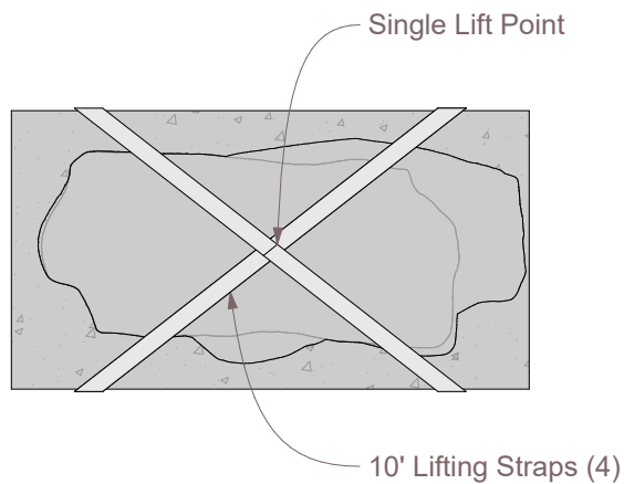
Pick Diagram - Plan
