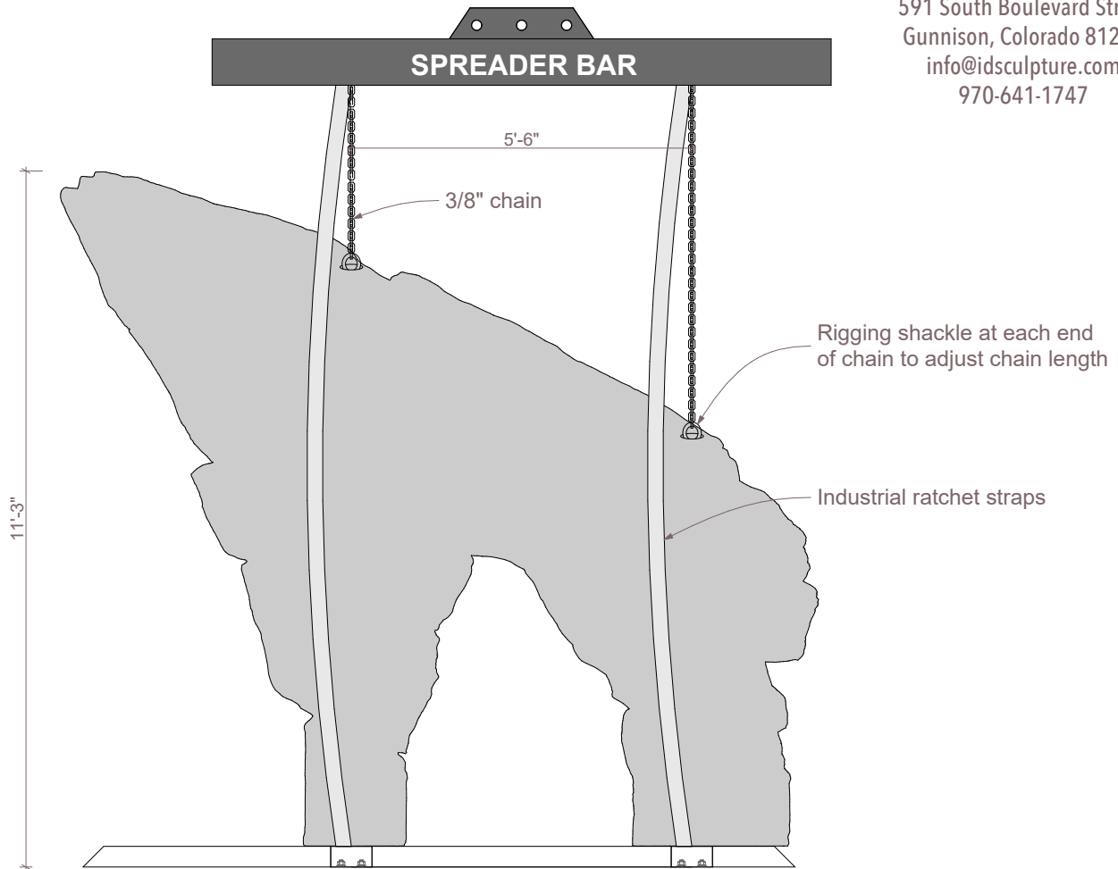
Rigging Diagram
