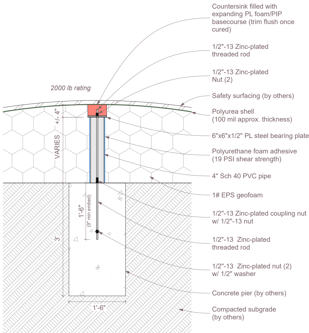
"Wet Set" Anchor Assembly - Detail
