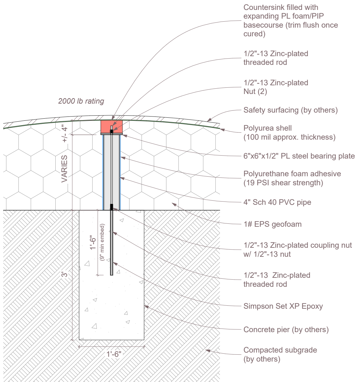
"Epoxy Set" Anchor Assembly - Detail
