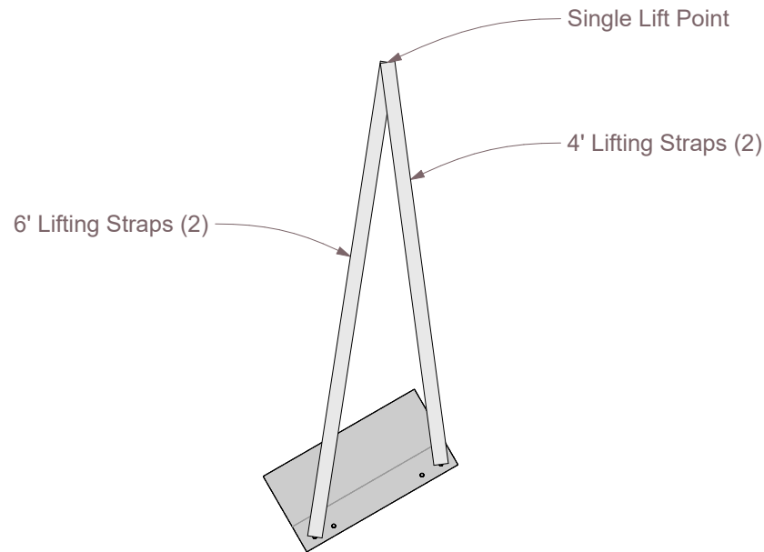
Slide Bed Module - Pick Diagram - Elevation
