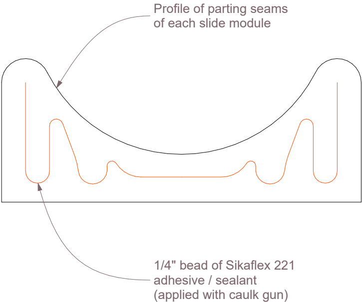
Slide Module Adhesive - Location Diagram
